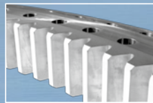
Slewing bearing with internal gear for a supply crane
